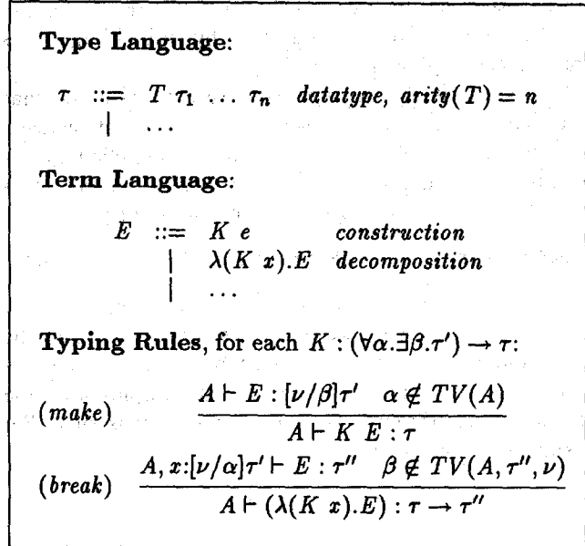
Figure 8: Extensions for FCP
