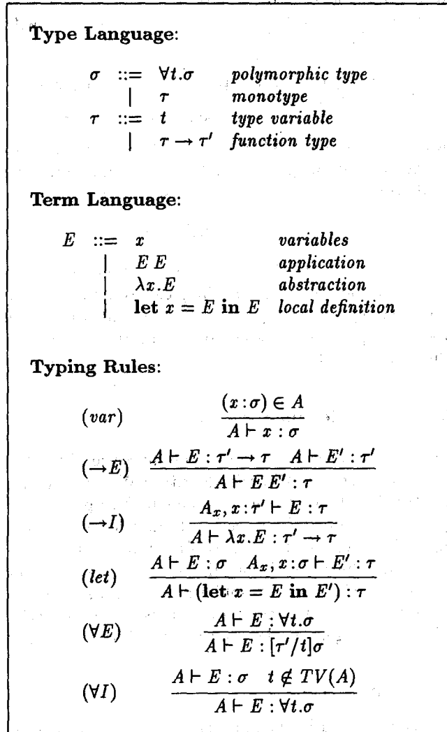
Figure 7: The Hindley-Milner Type System
